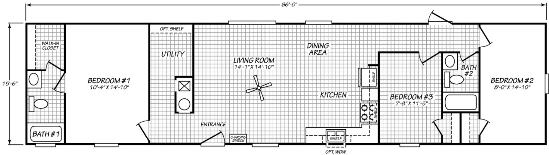
FLOOR PLAN 4 3 BEDS - 2 BATHS | 1023 SQ.FT.
